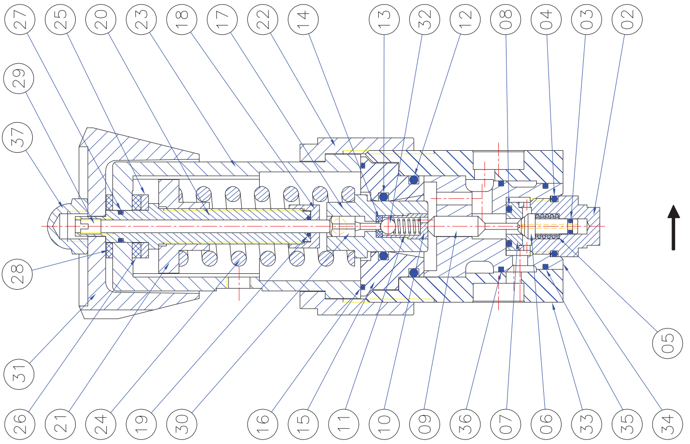
D104 pressure reducer
